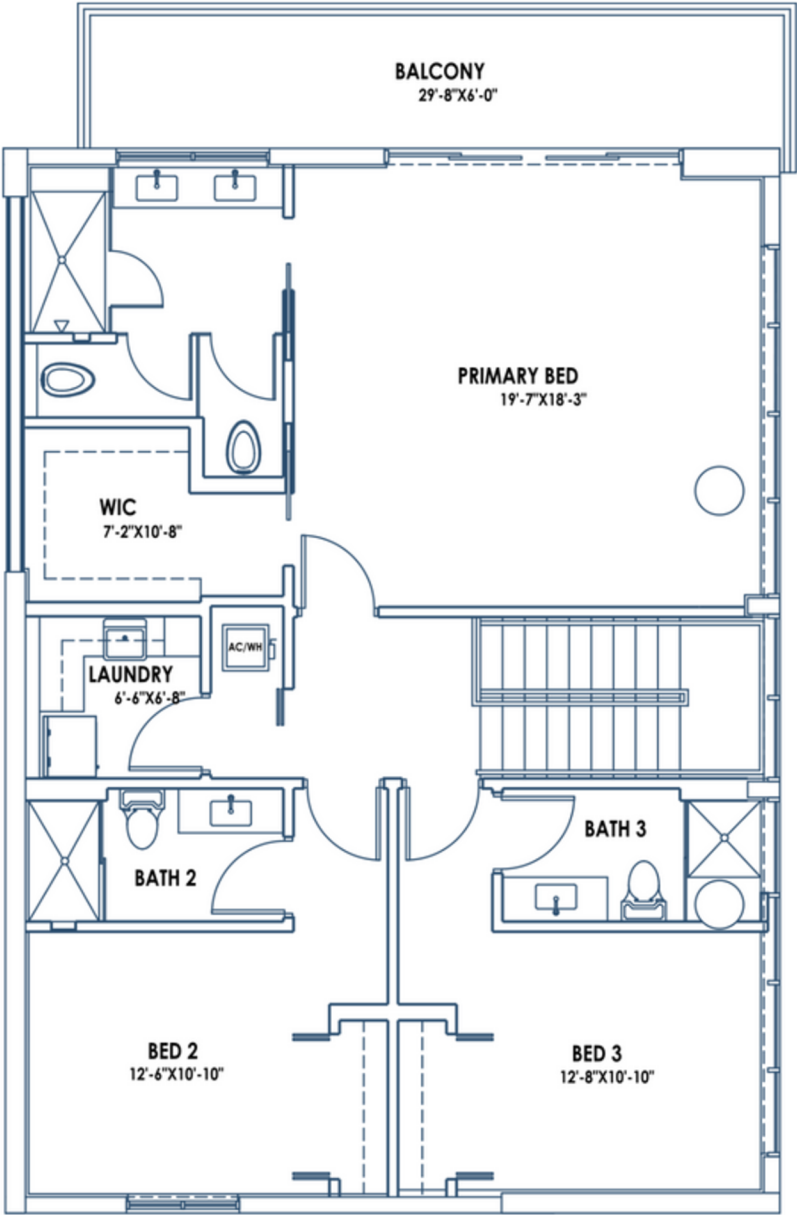
Top Floor
